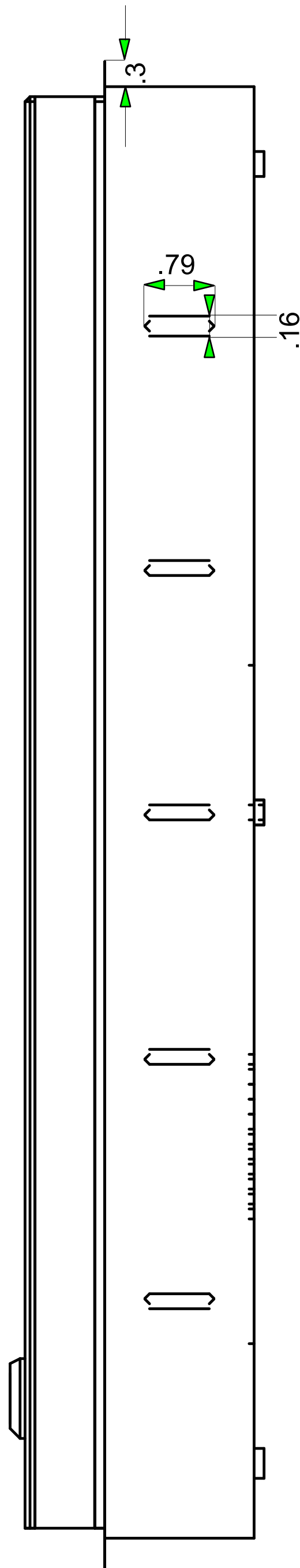
RIGHT VIEW
