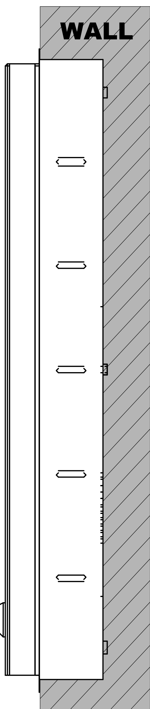
SIDE VIEW FLUSH MOUNTED ON WALL
