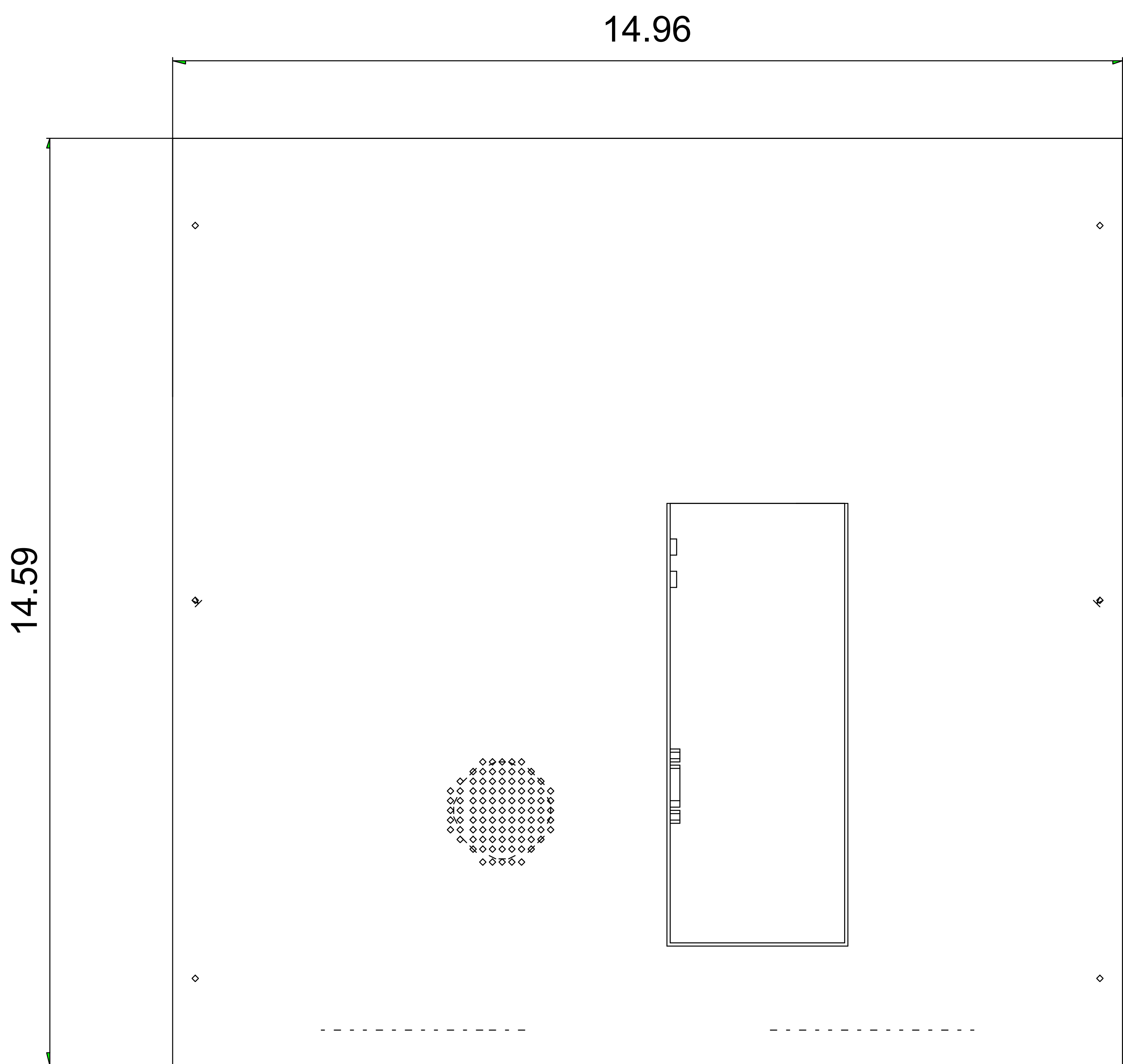
BACK VIEW
