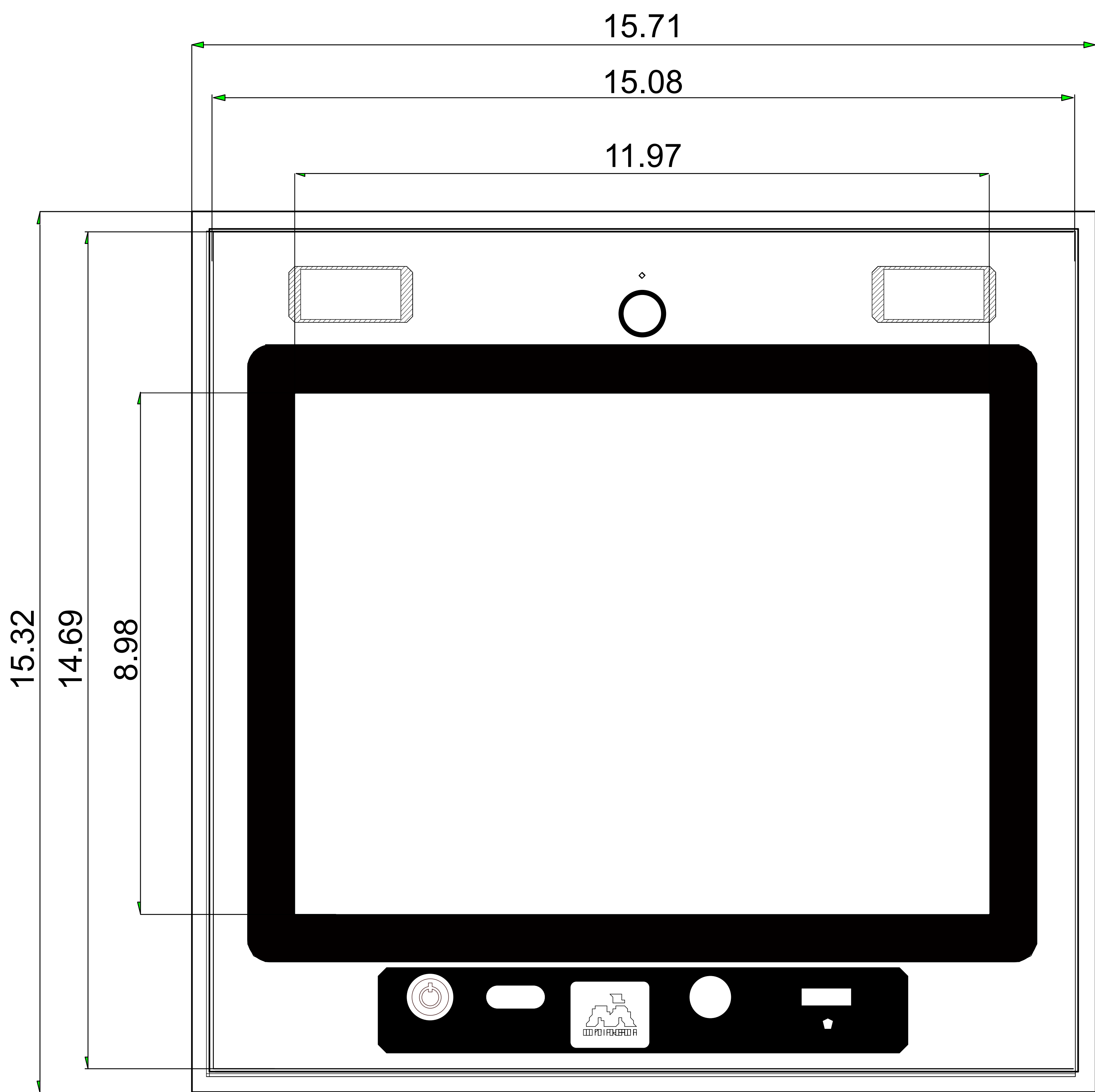
FRONT VIEW
