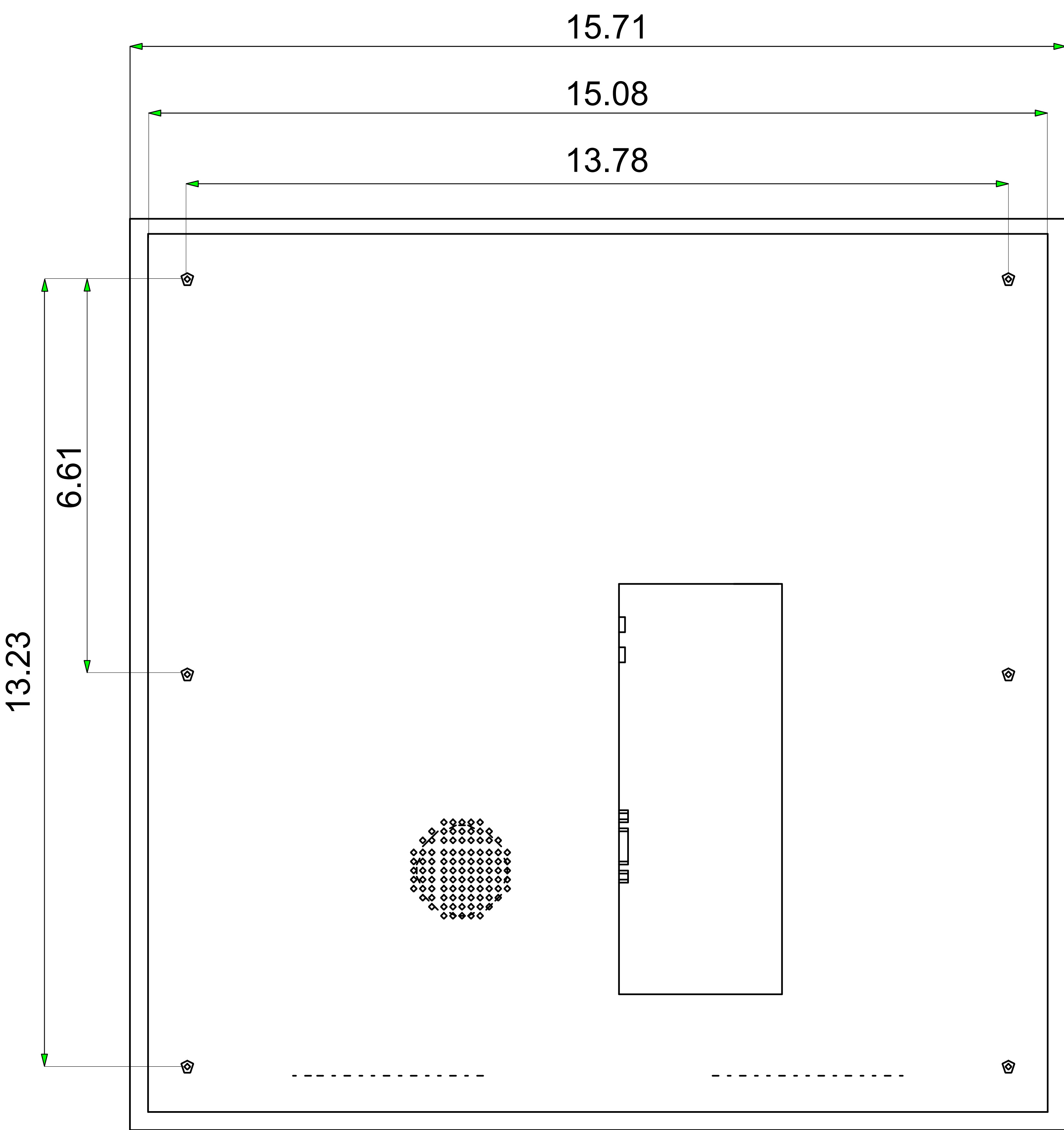
BOTTOM VIEW
