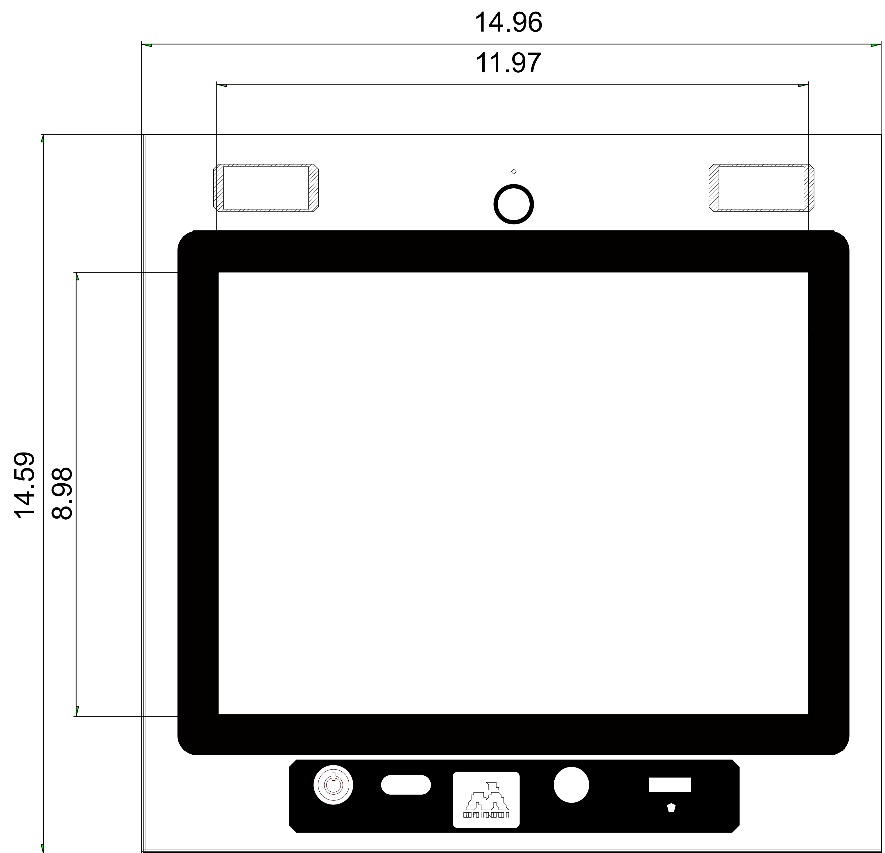
FRONT VIEW
