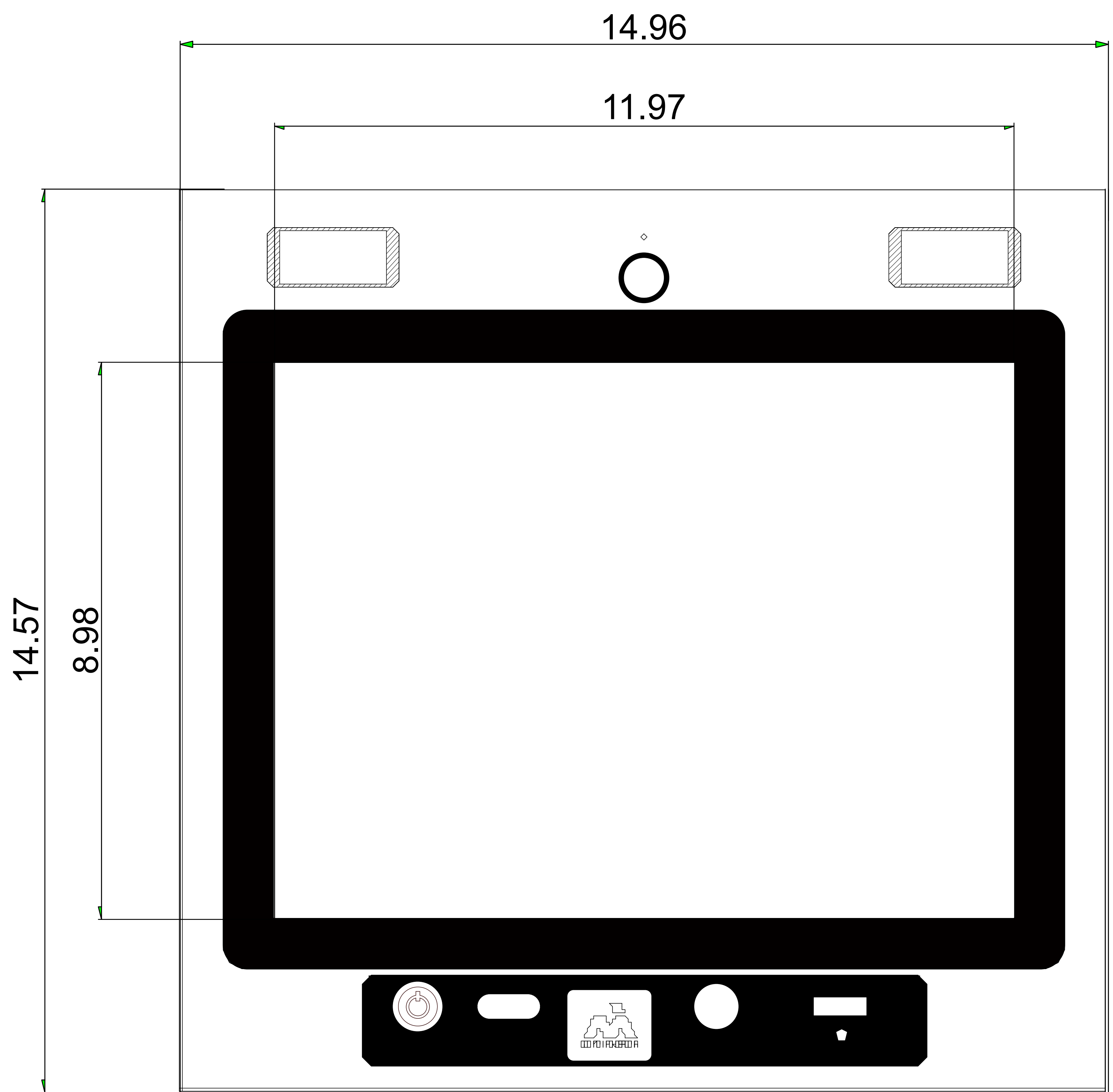
FRONT VIEW
