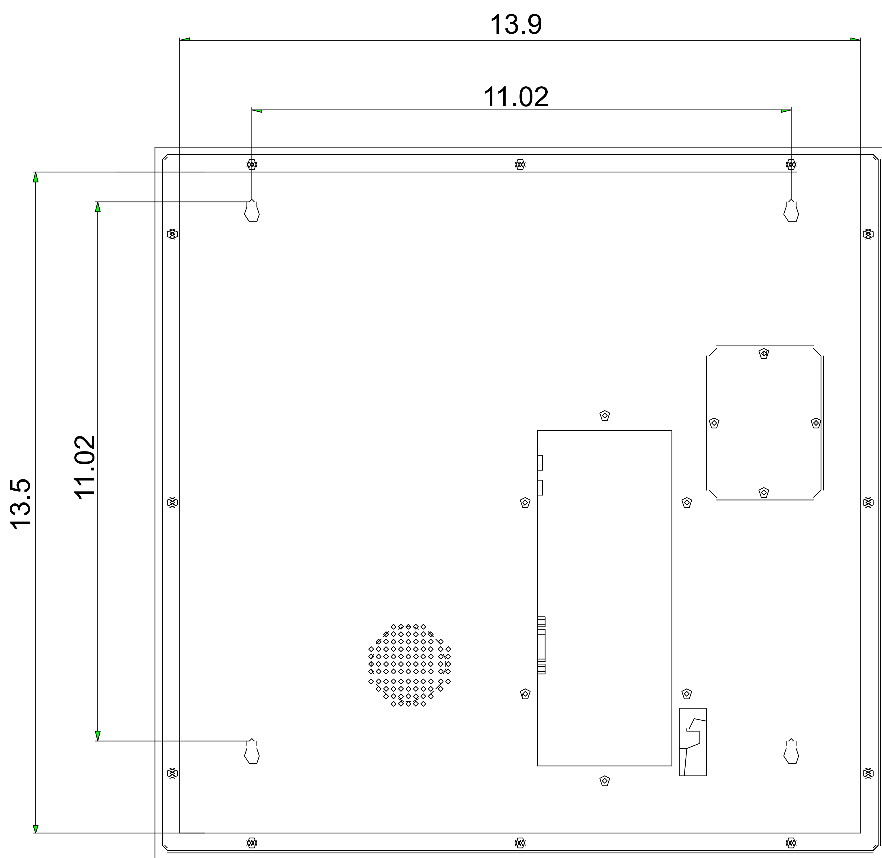
BACK VIEW
