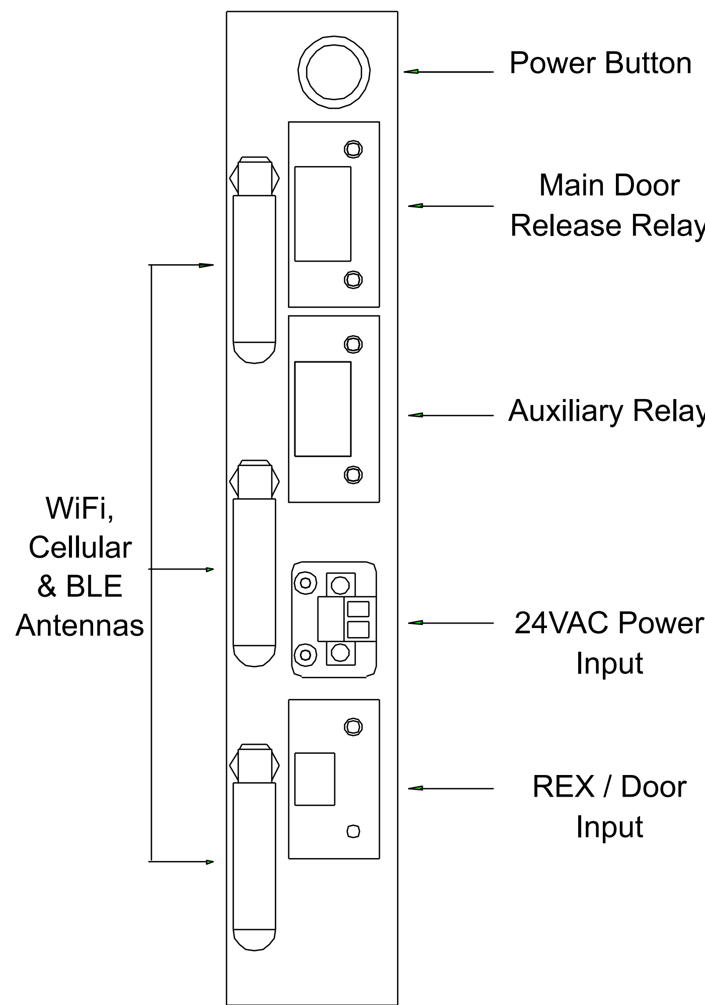
I/O PORTS (Right Side) (Ethernet Input & SIM Card Slot Not Shown)
